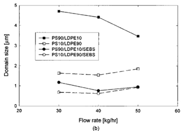
Fig. 3. Effects of SEBS compatibilizer for PS/LDPE blend on the domain size according to screw speed. (a) and flow rate, (b) in twin screw extrusion at 200 °C
