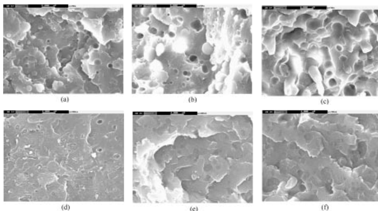
Fig. 1. SEM pictures of PS/LDPE blends and PS/LDPE/SEBS blends mixed by Haake Mixer at 100 rpm and 200 °C ( \times 2,000 ). (a) PS 90%, (b) PS 80%, (c) PS 70% (d) PS 90%/SEBS, (e) PS 80%/SEBS, (f) PS 70%/SEBS
