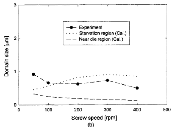
Fig. 5. Comparison between calculated and experimental domain sizes according to screw speed. (a) PS90%/LDPE10%/SEBS, (b) PS10%/LDPE90%/SEBS
