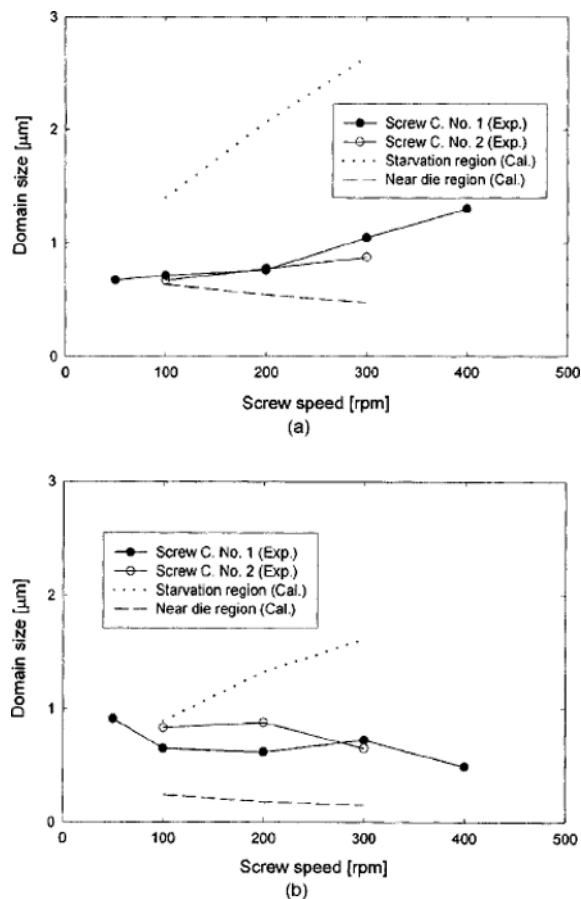
Fig. 10. Comparison between calculated and experimental domain sizes according to screw speed or different screw configurations.
