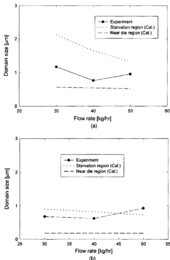
Fig. 6. Comparison between calculated and experimental domain sizes according to flow rate.
